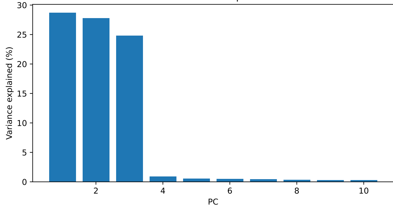
PCA: variance explained
